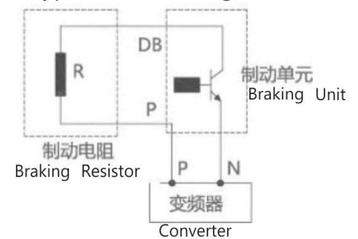
典型电路图 Typical Circuit Diagram
